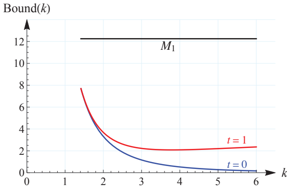
Figure 1: Bounds obtained by Theorem 1 when \sqrt{2} \leq k \leq 6 : Case (a) for t = 0 and t = 1
